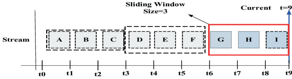
Figure 1. Example of sliding window sampling.
