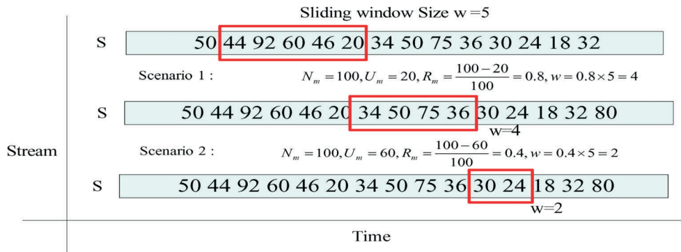
Figure 4. Example of window size adjustment.
