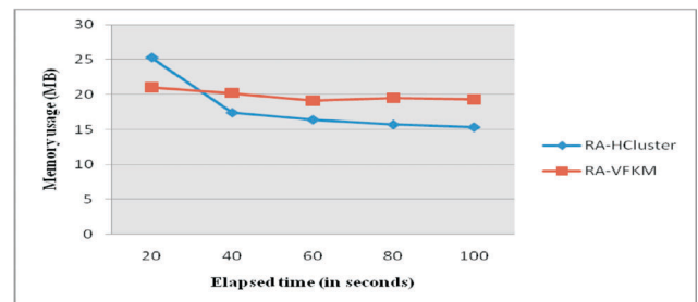
Figure 12. Comparison of memory usage by execution time.
