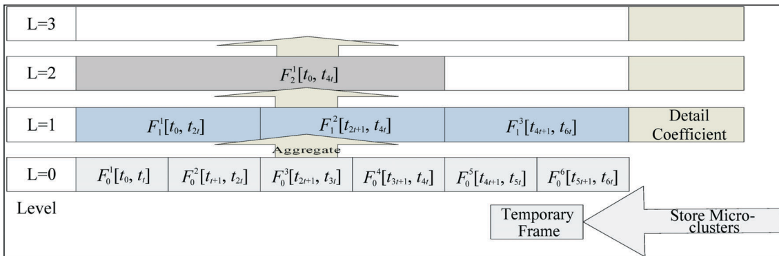
Figure 2. Hierarchical summary frame.
