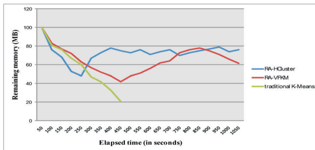
Figure 10. Comparison of memory usage.
