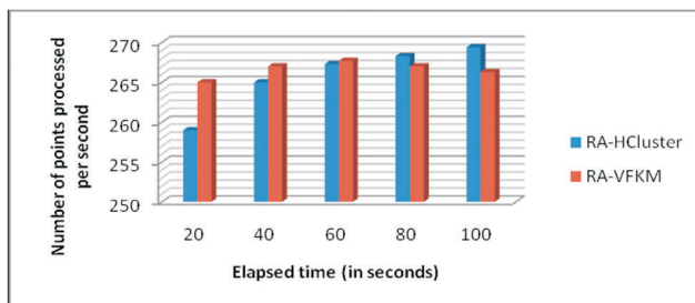
Figure 7. Comparison of stream processing efficiency for a longer elapsed time.
