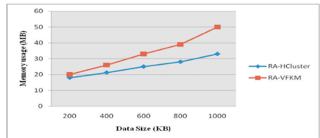
Figure 11. Comparison of memory usage by data size.
