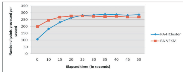
Figure 6. Comparison of stream processing efficiency.
