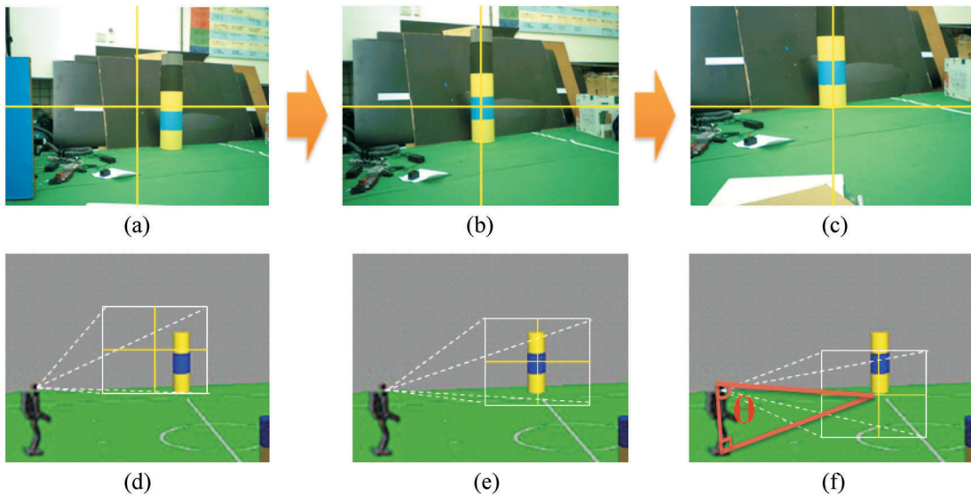
Figure 4. The images recognized by the robot through the CCD camera. (a)–(c) show the procedures of the robot to search the characteristic point and move the vision angle toward the object. (d)–(f) show how the robot head and CCD camera move.
