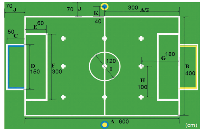
Figure 11. Configuration of the RoboCup soccer field for humanoid kid-size in 2009 [5].
