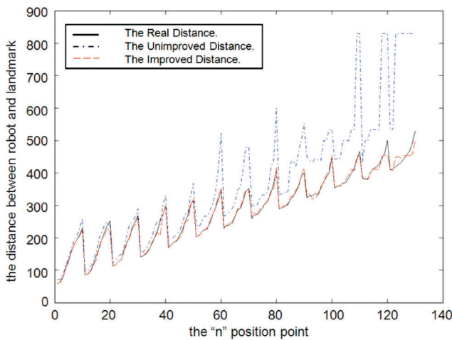
Figure 16. The error rates of the distance between the original and the improved approaches.
