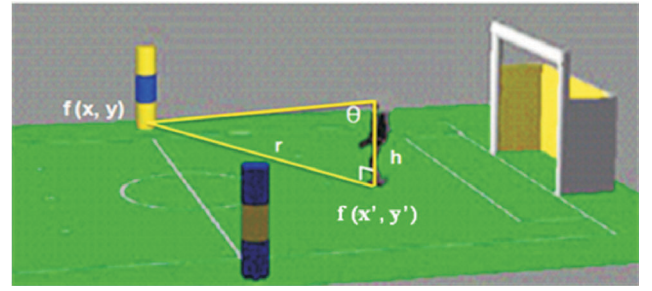
Figure 5. The relationship of r , \theta , h , f(x, y) and f(x', y') between the robot and landmark.
