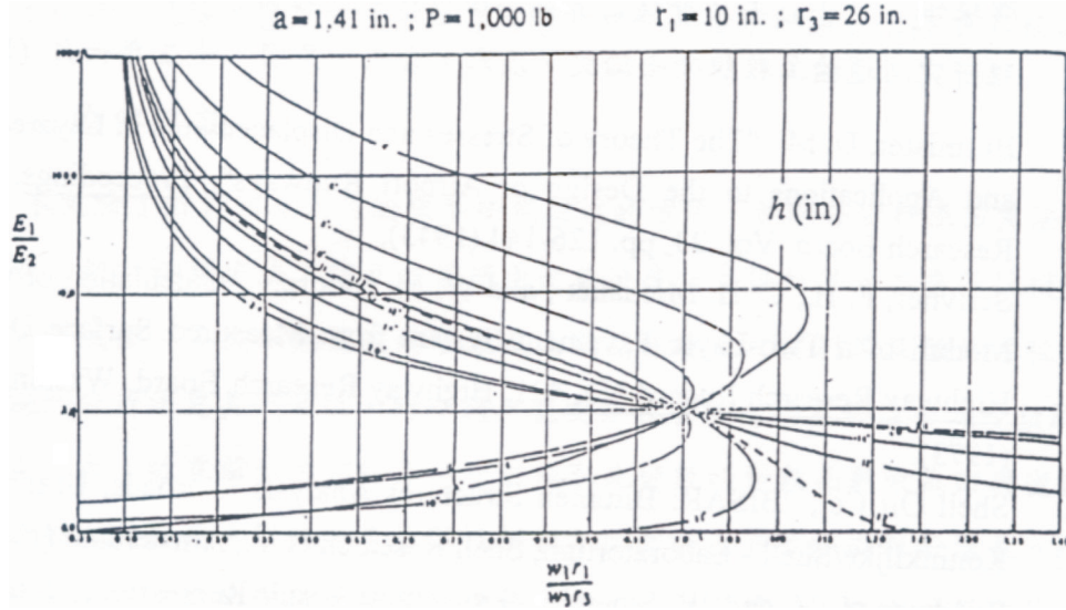
Figure 1. Scrivner's curves for two-layer backcalculation [6].
