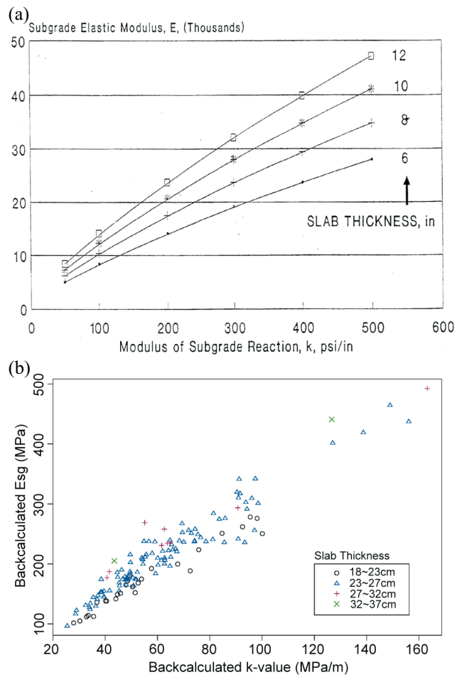
Figure 6. Comparison of elastic solid foundation versus dense liquid foundation based on: (a) theoretical comparison [25]; and (b) backcalculated results.
