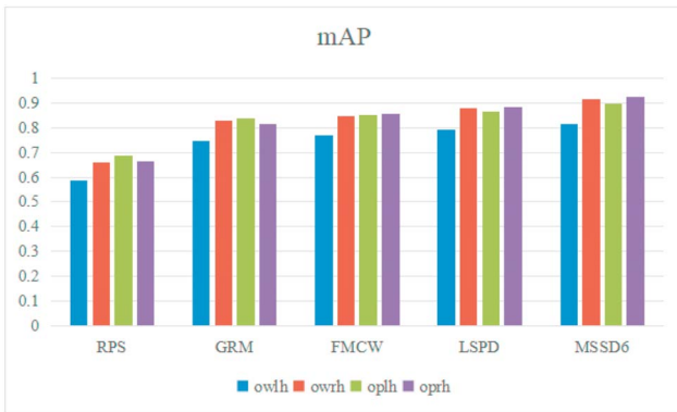
Figure 6. Four hands' mAP value.
