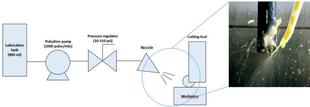
Fig. 2. Pulsating lubrication experiment strategy.
